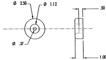
B1001 - 2.5" Round Rubber Bumper
