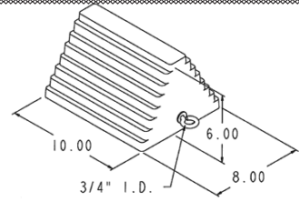
WC1468 - Rubber Wheel Chock
